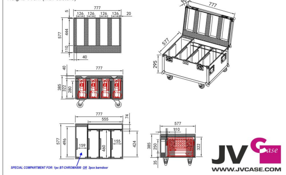
CASE FOR 4x BT-CHROMA800 External dimensions (incl ball corners): 80x60cm Height: 53cm (incl. castors)
