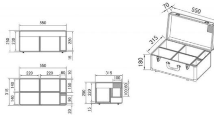
Flight case for 4 x COB-PLANO projectors + LEDCON-02 controller External Dims.: 550*315*250mm
