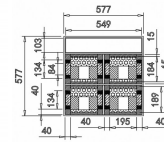
Flightcase for 4x EXPLORER SPOT EXTERNAL DIM: 577 x 577 x 490 mm (with ball corners: 60 x 60cm standard size)
