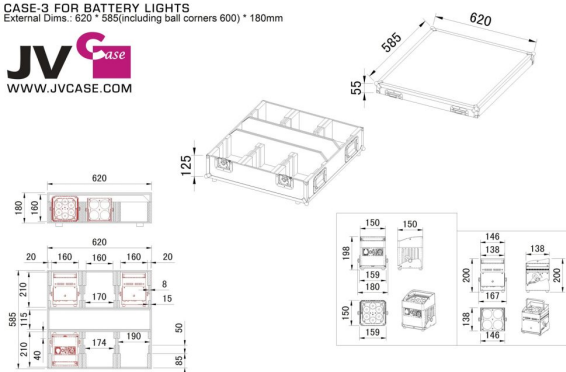
CASE-3 FOR BATTERY LIGHTS External Dims.: 620 * 585 (including ball corners 600) * 180mm
