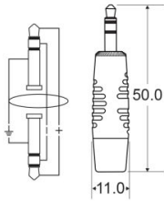
REAN® Jack connectors
