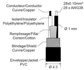
High Performance Line Cable 0.22 mm 2 / 28 x 0.10 mm / AWG 24
