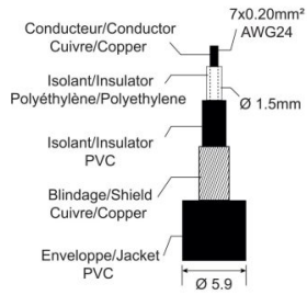
High Performance Microphone Cable 0.22 mm 2 / 28 x 0.10 mm / AWG 38
